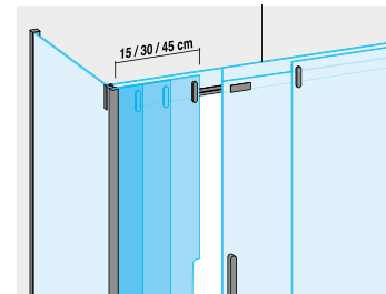
DOOR + FIXED SIDE MOD. WITH HANDLE ON THE LEFT, FIXED SIDE IN LEFT CORNER
