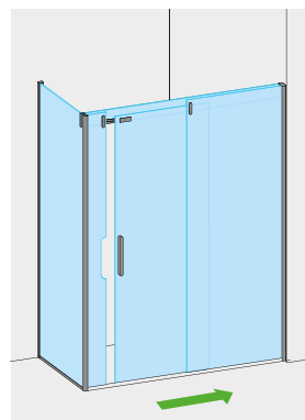
DOOR + FIXED SIDE MOD. WITH HANDLE ON THE LEFT, FIXED SIDE IN LEFT CORNER
